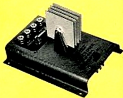
No. 32654 Rectifier. Changes AC from transformer to low voltage DC for train operation. 3 amp. output. Has reset type circuit-breaker 3 3/8" high, 4 5/8" wide, 6 1/4" long... $7.98
