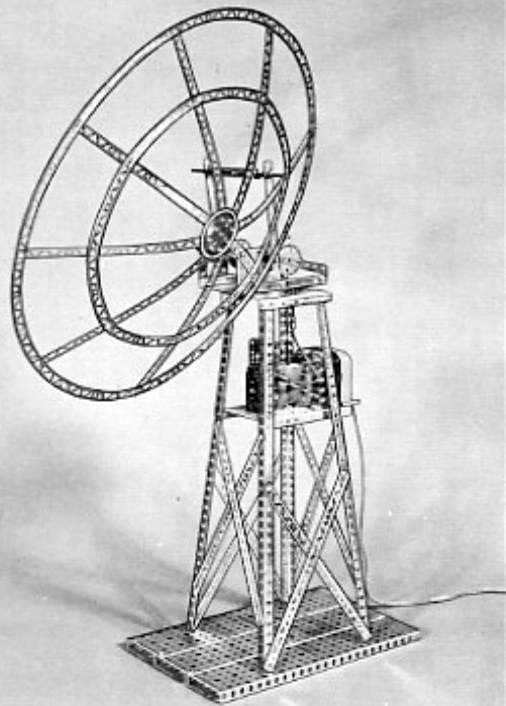
No. 17034 Giant Satellite Tracker. Dramatizes how well Erector fits into space age technology! Big 20" "dish" antenna rotates 360° and rocks up and down in realistic scanning motion as it turns—a real eye-catcher on counter or in window. 32" high, base 12½" x 8". Shipping weight 12 lbs. $14.50 NET
