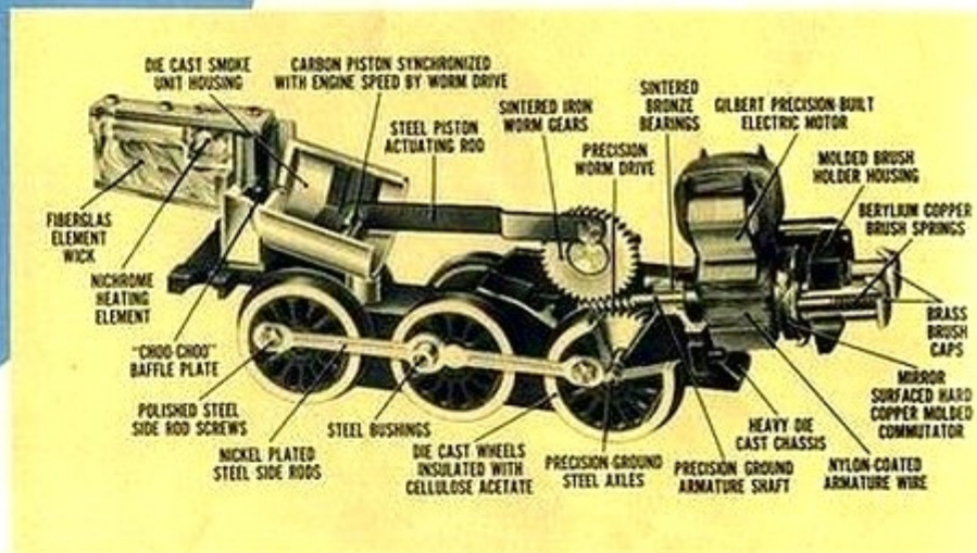
Photograph above is a close-up of the American Flyer No. K325 Hudson illustrated on pages 13 and 18.
