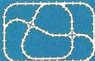
No. 16—Space 80" x 120" Track 28 Curve 30 Straight 3-1/2 Straight 2 pair of Switches 2 Crossovers
