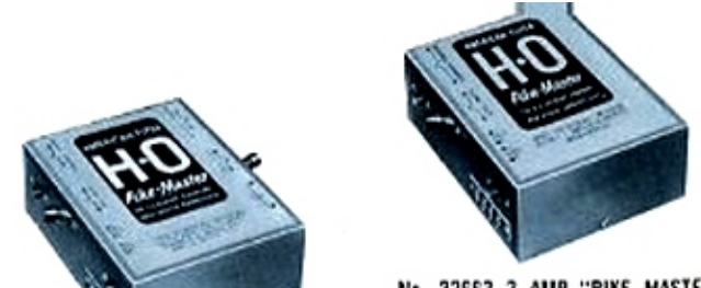
No. 32652 2 AMP "PIKE MASTER" POWER PACK — Reduces 110-120 volt A.C. household current to 12 volts D.C. for train operation and to 16 volts A.C. for accessories. Built-in thermostatic circuit breaker guards against shorts and overloads. Throttle control and reversing switch. 12.98
